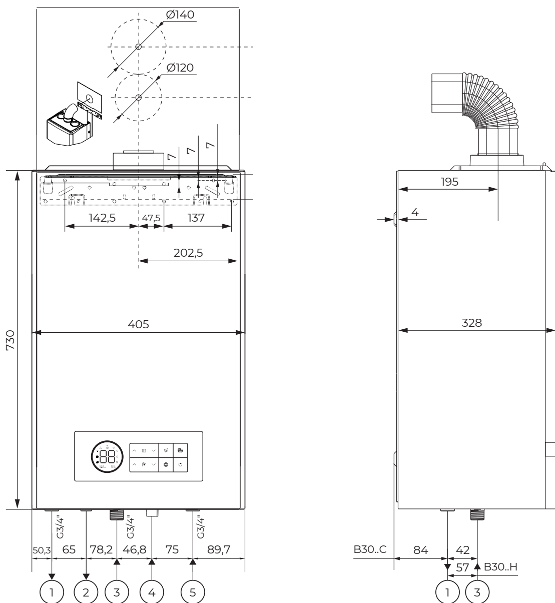
Рис. 43. B30 28 C/H, B30 32 C/H, B30 36 C/H.
